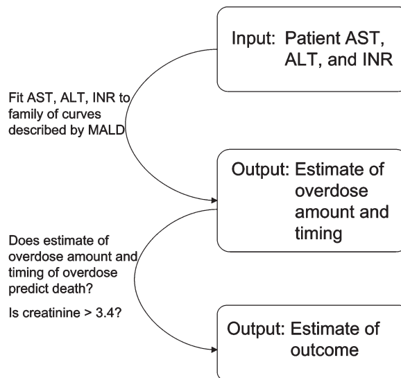
Fig. 4. A schematic description of how MALD can be used to estimate overdose amount, timing, and outcome. Patients' AST, ALT, and INR are fit to a family of curves described by MALD to estimate overdose amount, timing, and outcome. If outcome is predicted to be poor, liver transplantation may be necessary.
