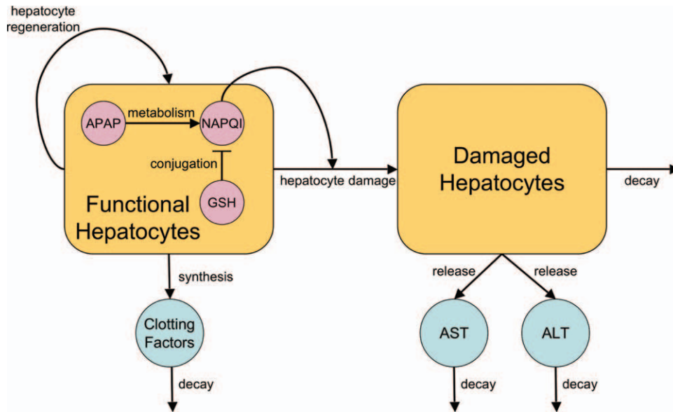
Fig. 1. A schematic diagram representing the dynamics of the mathematical model. A fraction of APAP is oxidized to NAPQI, bound to GSH, and safely eliminated. As GSH stores are depleted, NAPQI damages hepatocytes, releasing AST and ALT into the blood. Meanwhile, functional hepatocytes regenerate and produce essential clotting factors. Red represents the intracellular variables, yellow represents healthy and damaged hepatocytes, and blue represents markers of liver damage.
