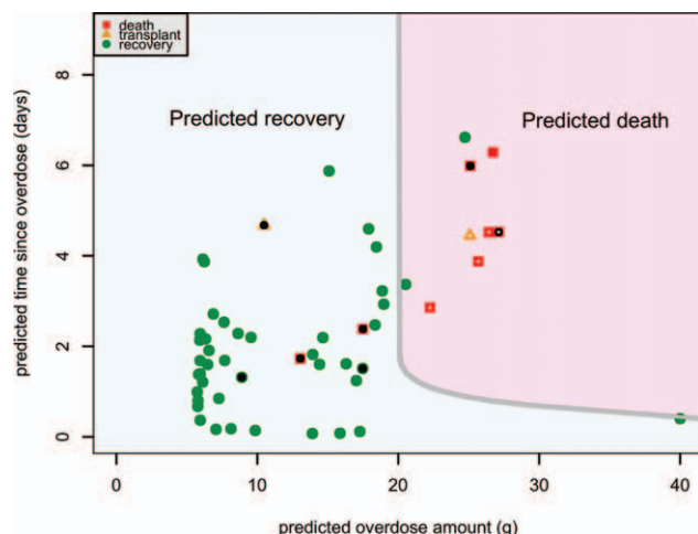
Fig. 2. MALD derived estimates of time since overdose and overdose amount for 53 patients with known APAP overdose. Red squares indicate eventual death, green circles recovery, and orange triangles transplant. Small white dots indicate \text{INR} > 6.5 and small black dots indicate serum creatinine > 3.4 mg/dL on admission. The gray line indicates overdose amounts and times since overdose for which 70% hepatic necrosis is predicted. Patients to the right and above the gray line are predicted to die.
