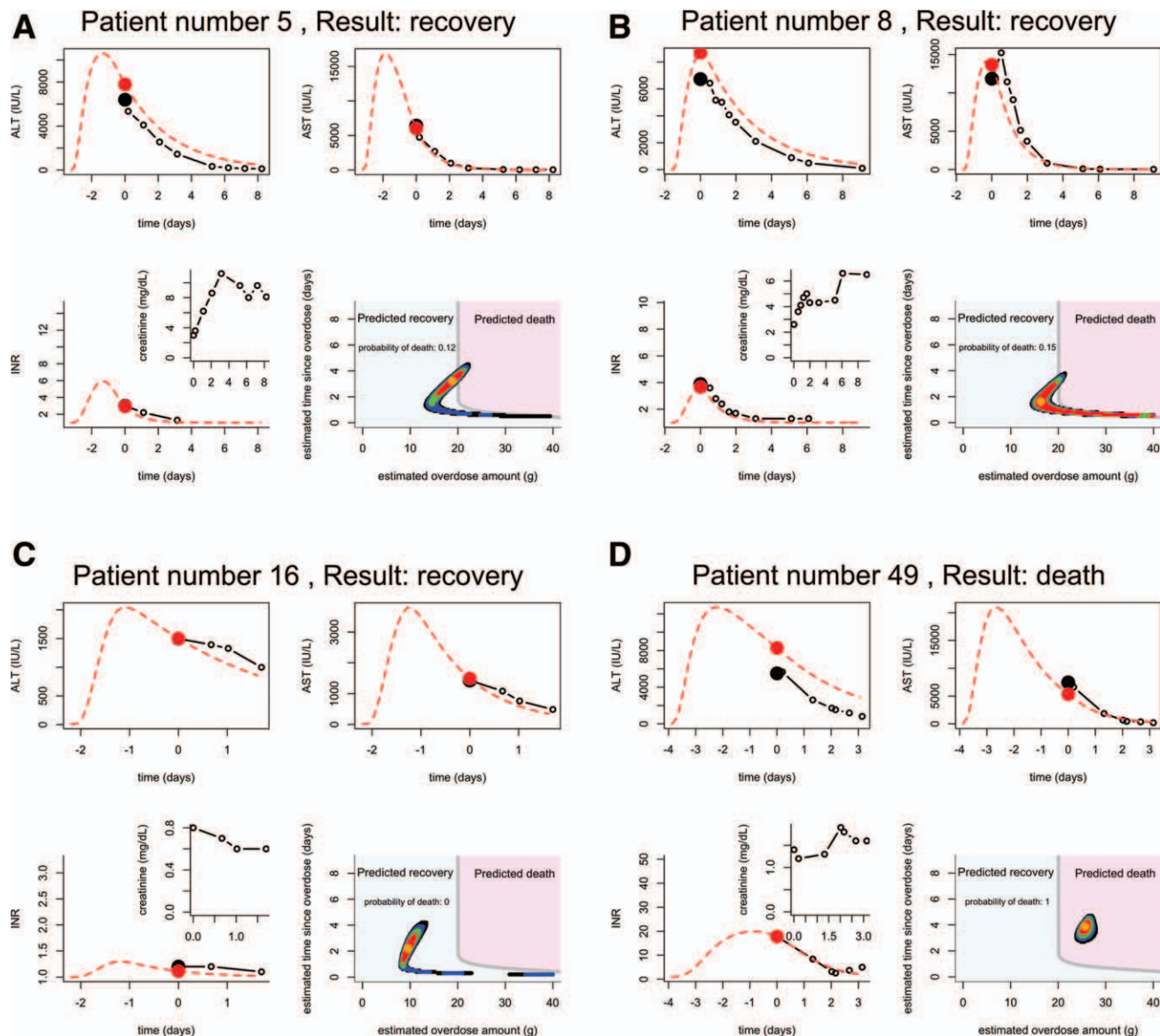
Fig. 3. Markers of liver damage (small black open circles) and model predictions (red dashed line) based on least squares fits of initial AST, ALT, and INR (large black filled circle) to modeled AST, ALT, and INR (large red filled circle) for four representative patients. Time t = 0 indicates the time of admission to hospital. The estimated overdose amount and time since overdose for each patient is given by the orange dot in the lower right panel. Refer to the Supporting Information for more details.
