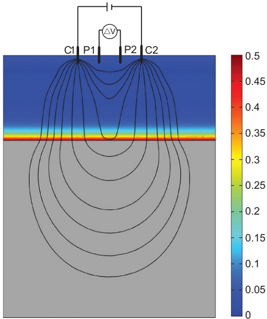
Fig. 2. A Wenner array with four evenly spaced electrodes, probing a sea ice floe of thickness 0.8 m, on top of sea water. The color scale indicates the value of the vertical conductivity of the sea ice in (\Omega \text{ m})^{-1} , calculated from a brine volume profile we measured in Antarctica, using F(\phi) = 8.6\phi^{2.75} . The horizontal conductivity is assumed to be 1/4 the value in the vertical direction. Comsol 3.5a was used to calculate the electric current streamlines. The conductivity of the sea water is 4.8 (\Omega \text{ m})^{-1} .
