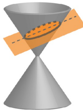
Ellipse
